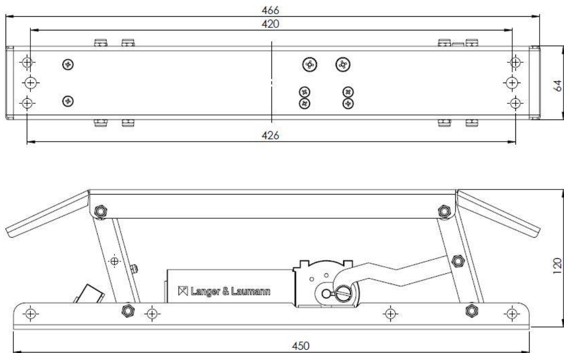
Fig. 3: Came mobile L&L ouverte
