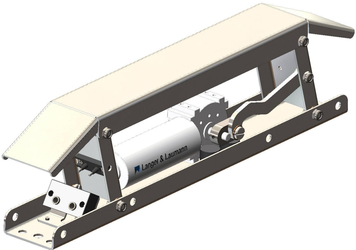
Fig. 2: Came mobile L&L ouverte
