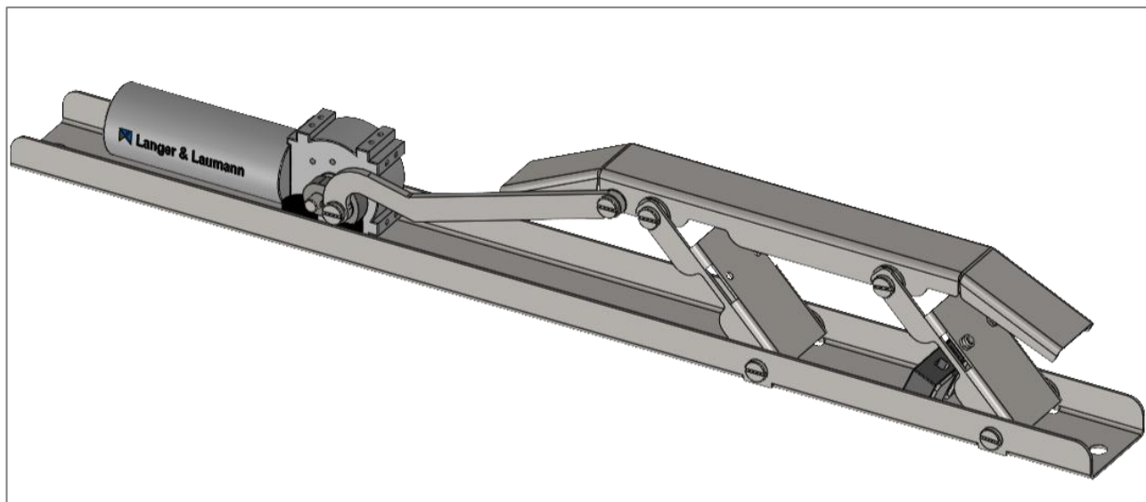
Fig. 1: Came mobile L&L fermée
