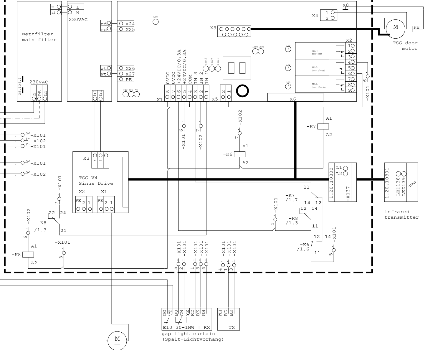
TSG Sinus Drive for moving interlock shaft door
