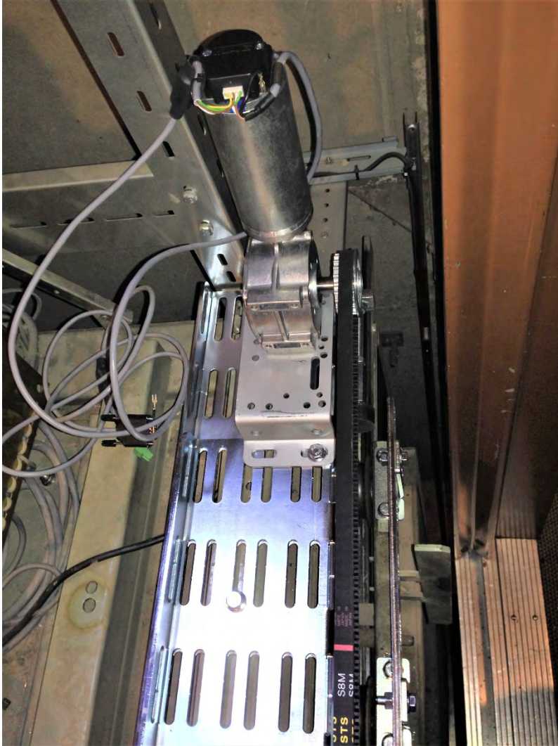
Fig. 9: TSG drive unit
