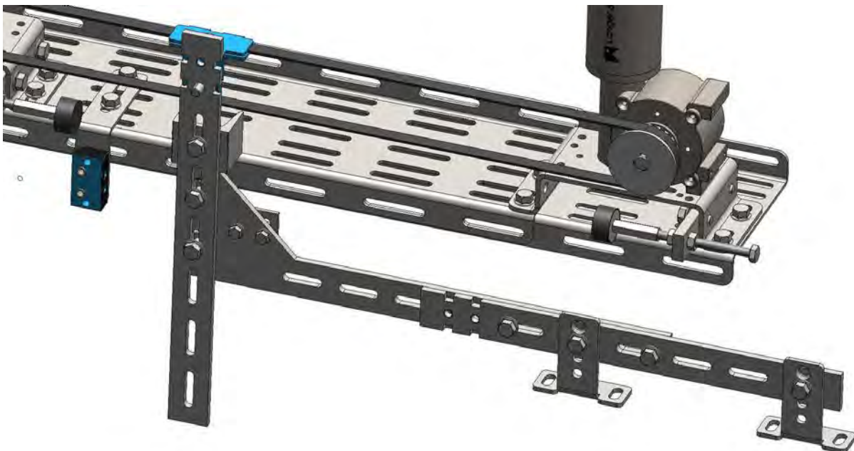
Fig. 6: TSG door panel coupler
