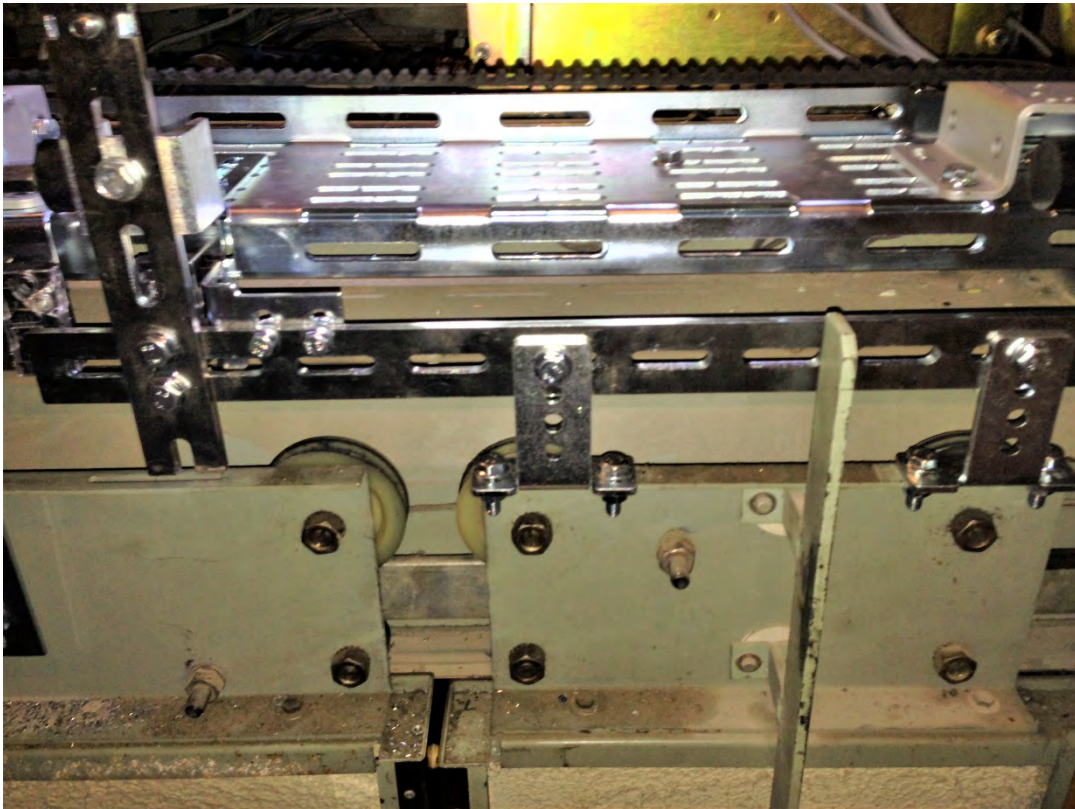
Fig. 5: TSG door panel coupler
